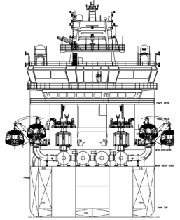
TRANSVERSE SECTION SATURATION SYSTEM
