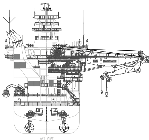
AFT VIEW
