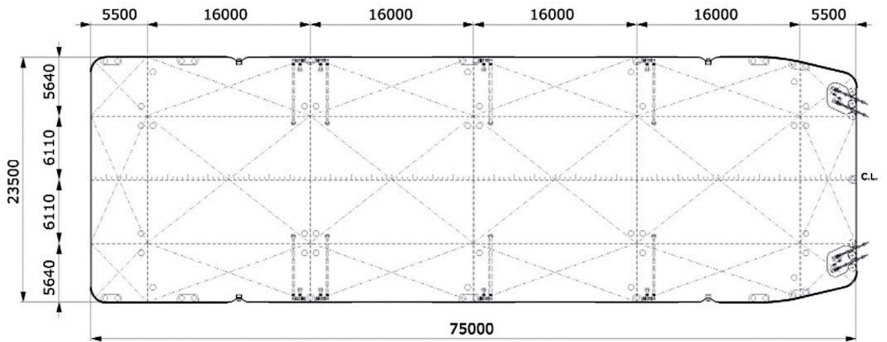
TOP VIEW DECK LEVEL
