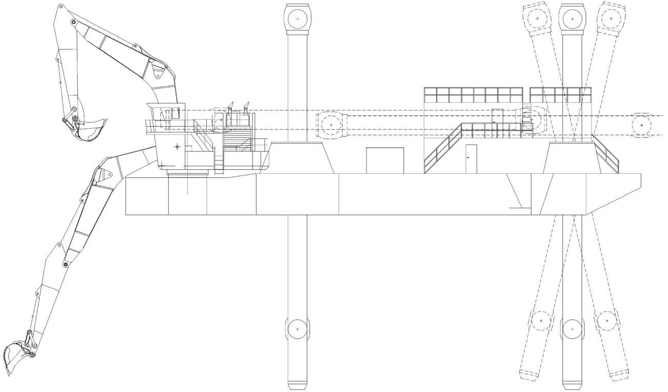
SIDE VIEW
