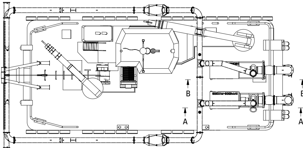
TOP VIEW DECK LEVEL
