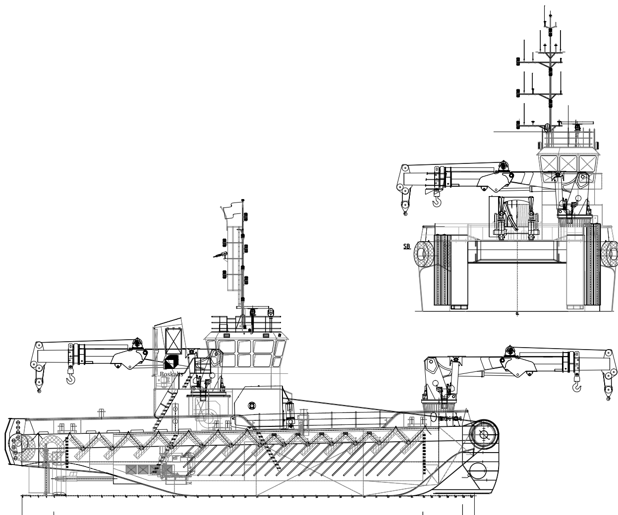
SIDE VIEW
