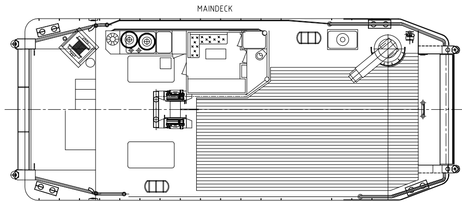
TOP VIEW DECK LEVEL
